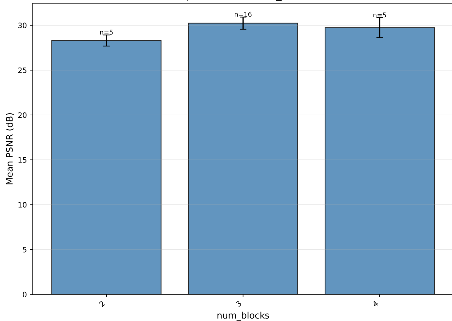
Mean PSNR per value of num_blocks — SwinT
